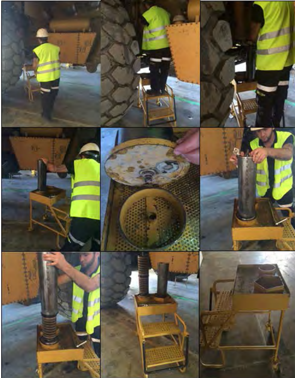
Practical use of Transmission and Hydraulic Filter Replacement Tool
