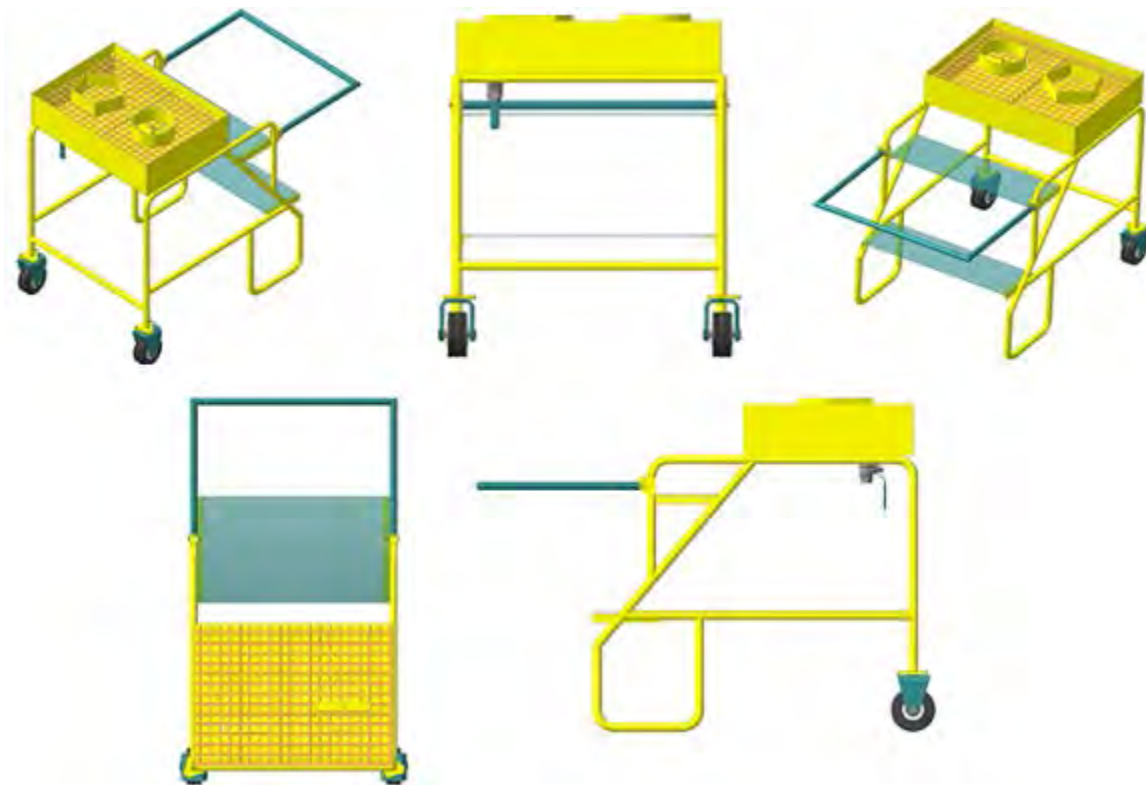
Transmission and Hydraulic Filter Replacement Tool pictures in 3D
